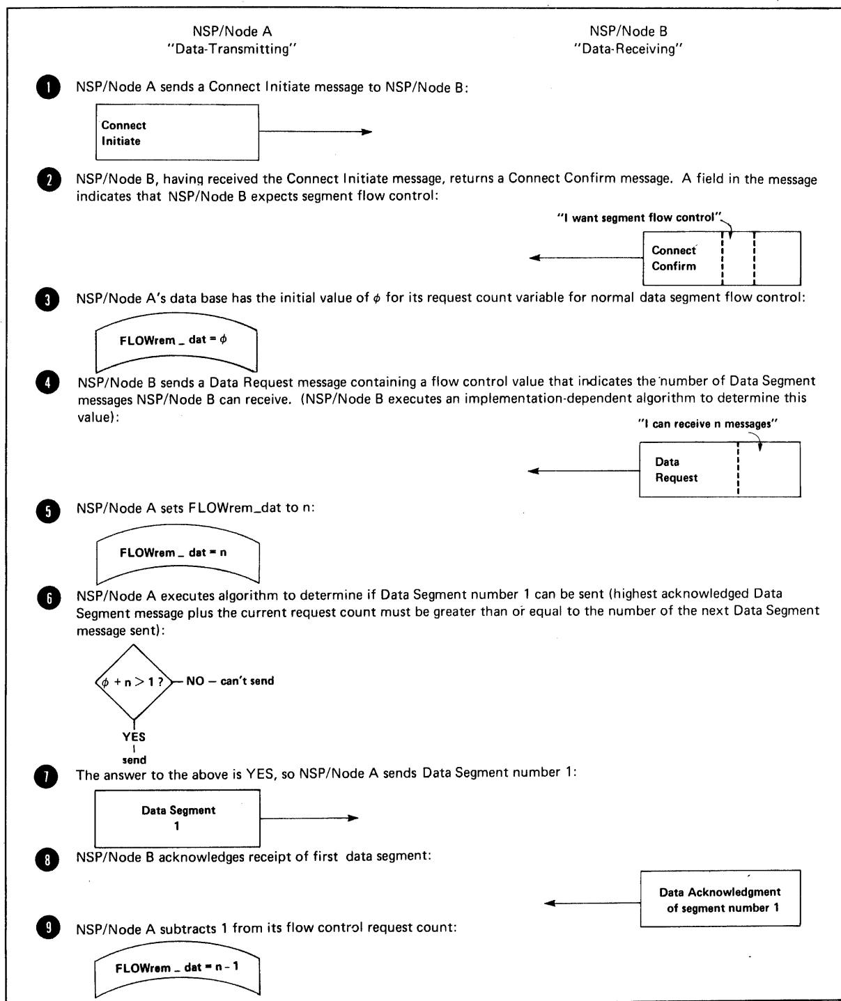
Figure 4-4: Segment Flow Control Shown in One Direction on a Logical Link
