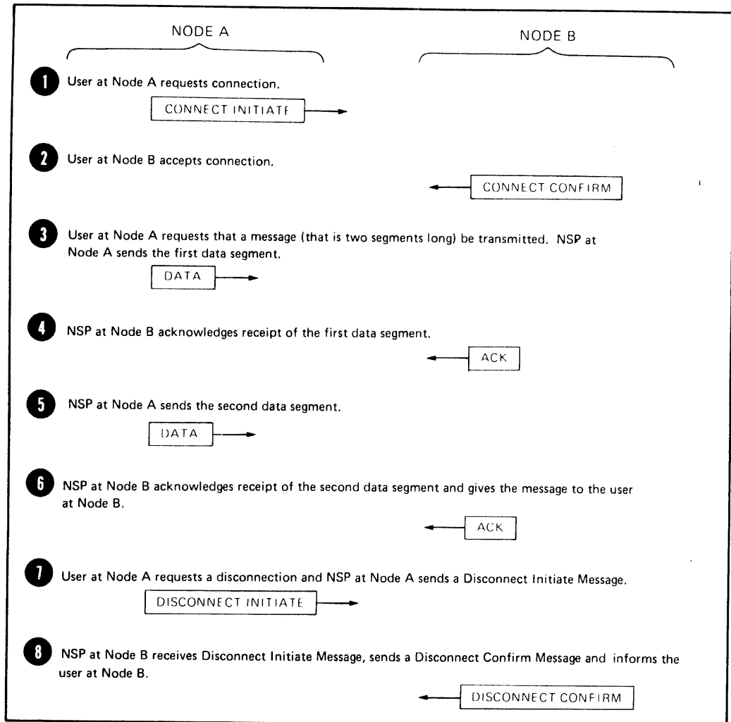
Figure 4-2: Typical Message Exchange Between Two Implementations of NSP
