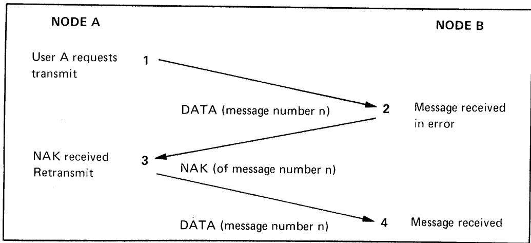
Figure 2-5: DDCMP Message Exchange, Showing Error Recovery
