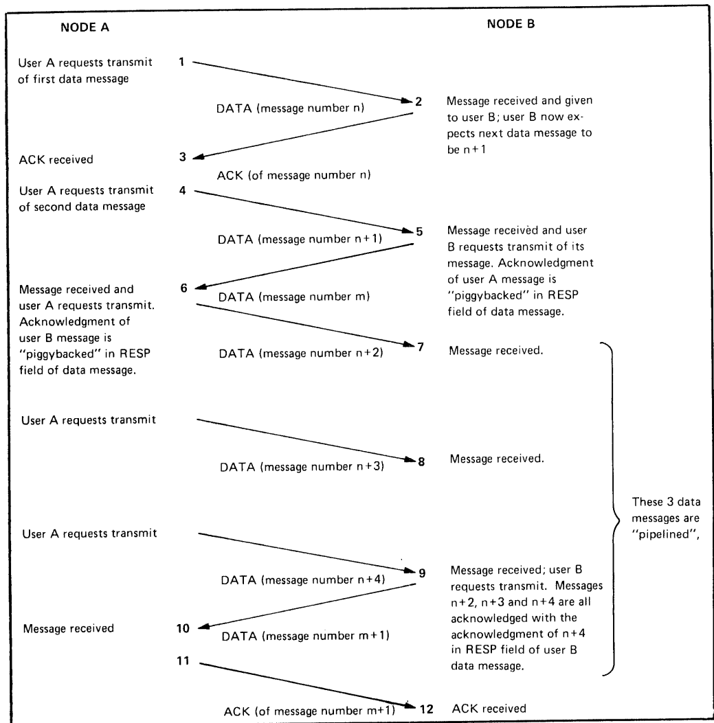
Figure 2-4: Typical DDCMP Message Exchange, Showing Positive Acknowledgment, Piggybacking, and Pipelining
