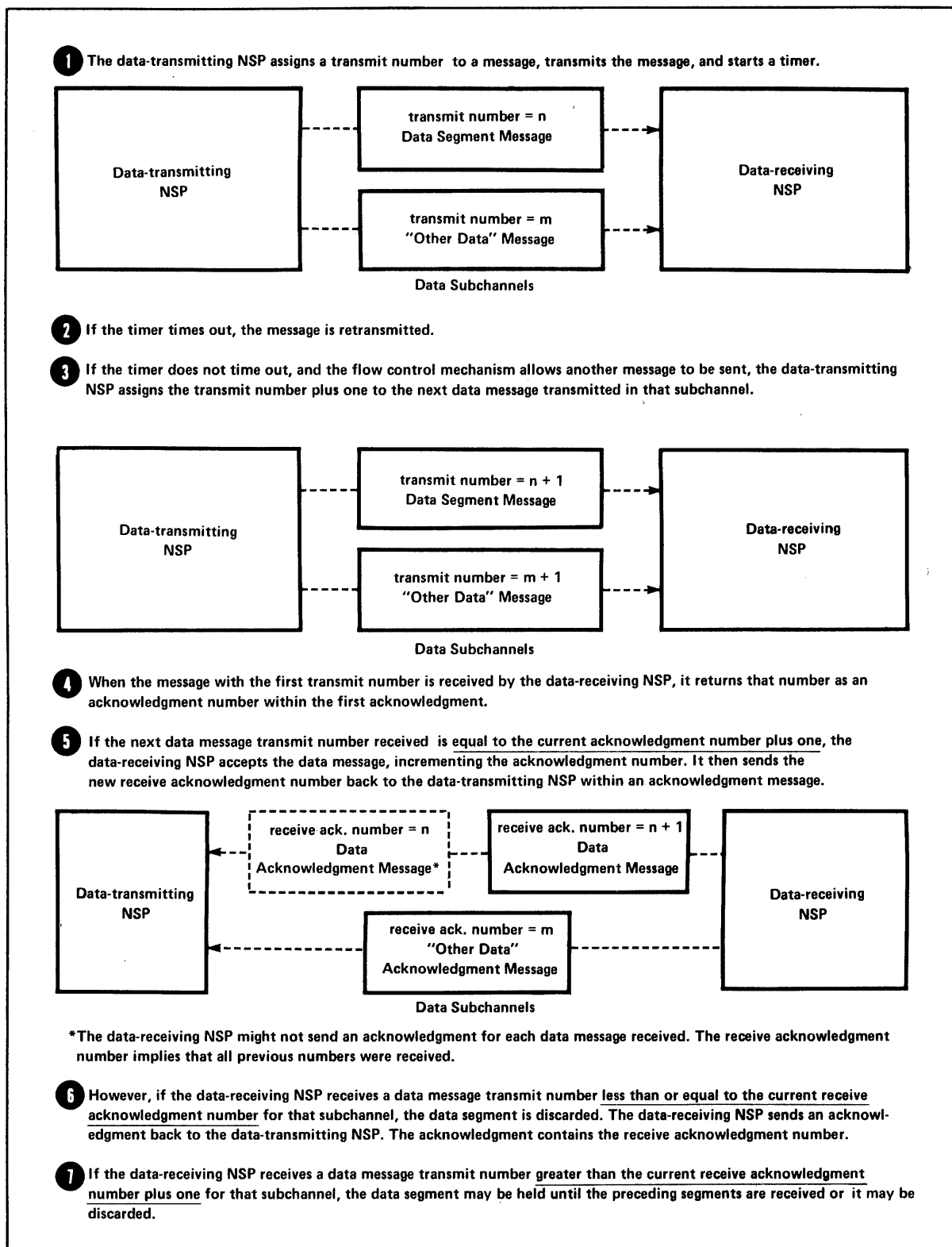
Figure 4-3: Acknowledgment Operation
