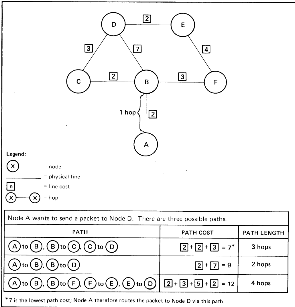
Figure 3-1: Routing Terms
