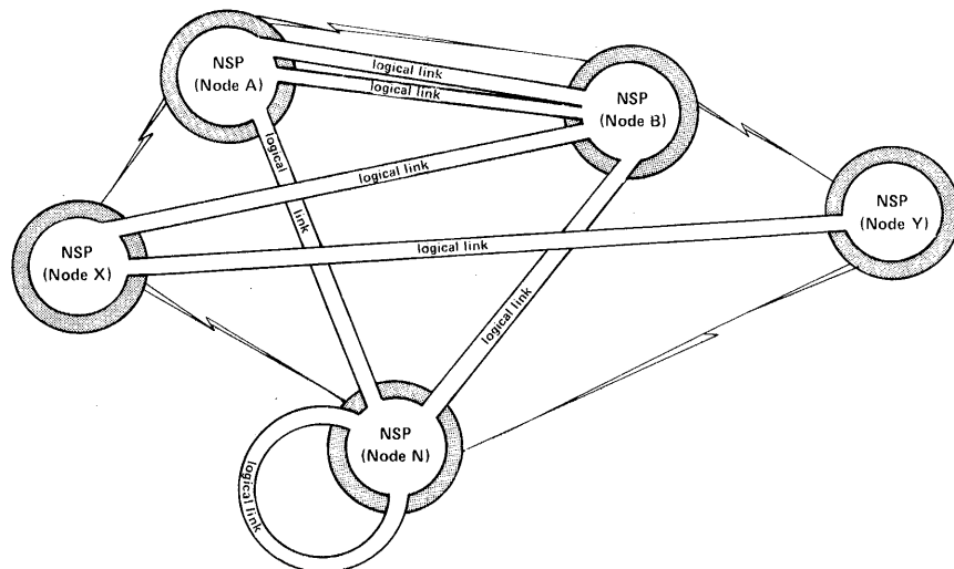
Figure 4-1: Logical Links
