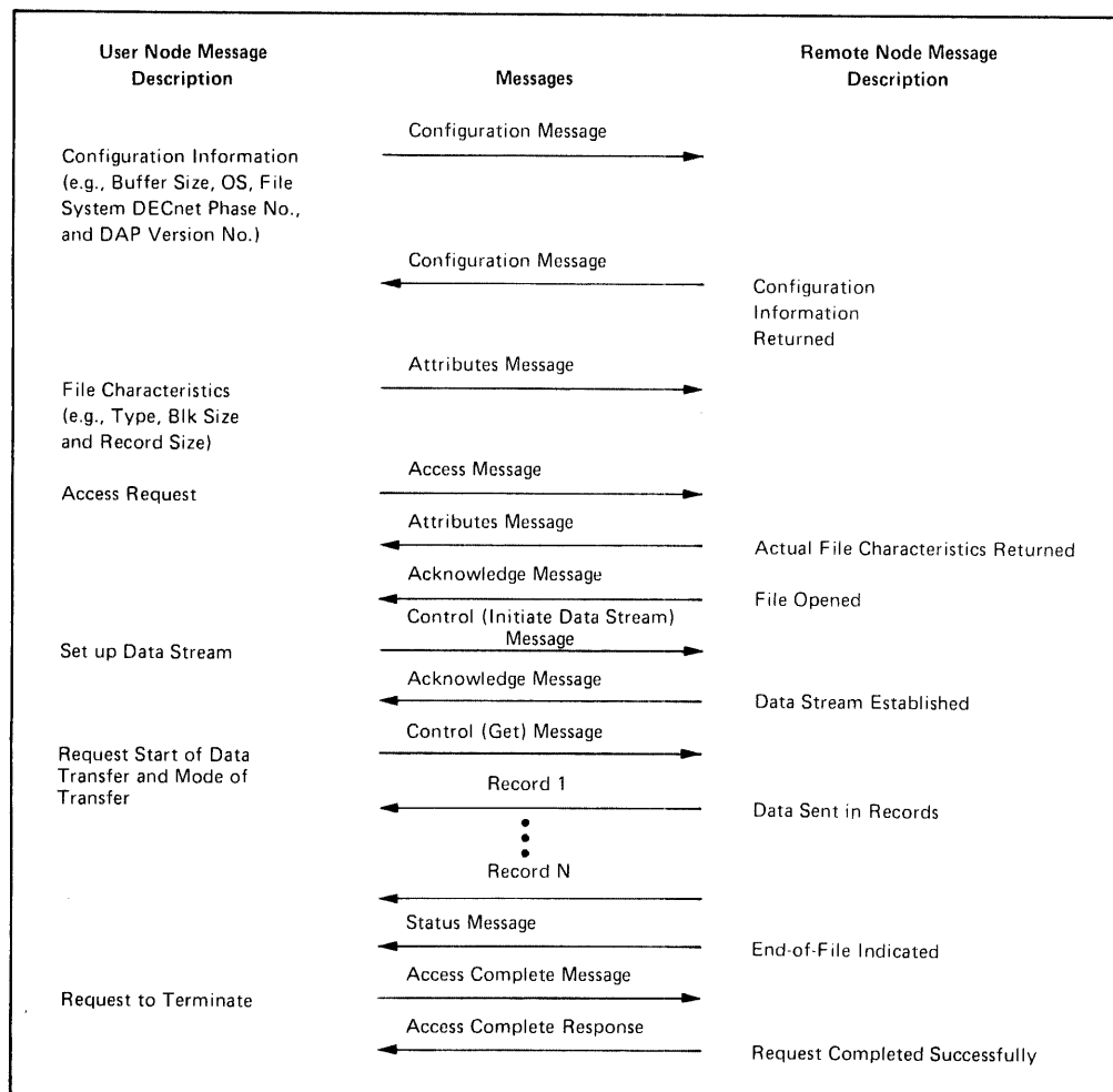
Figure 6-1: DAP Message Exchange (Sequential File Retrieval)
