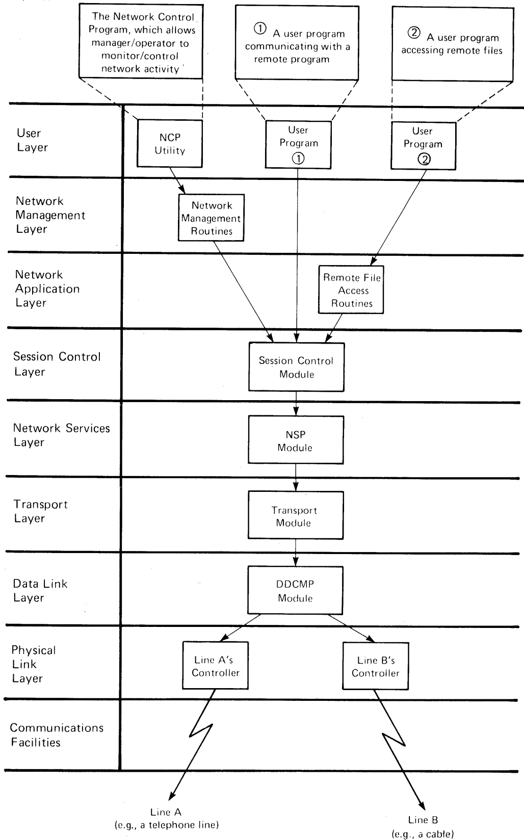
Figure 1-3: DNA Modules Resident in a Typical DECnet Node
