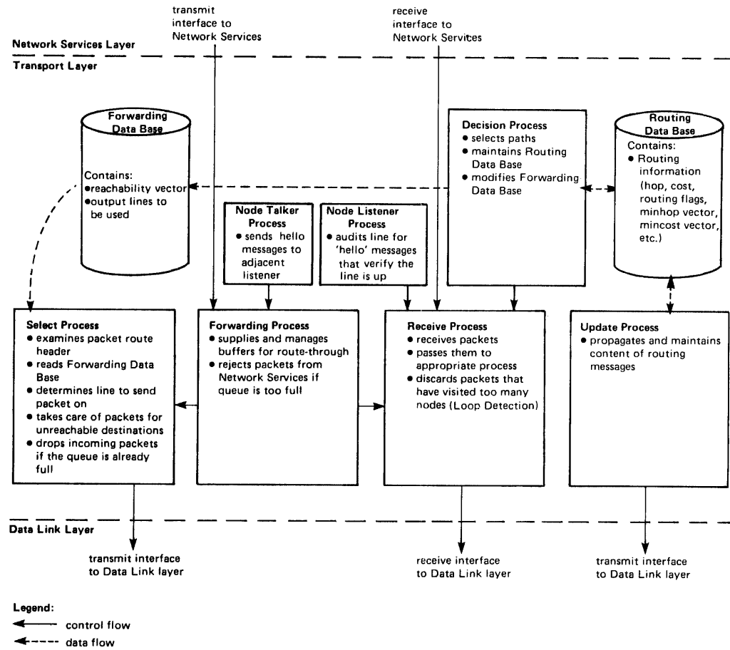
Figure 3-4: Transport Control Components and their Functions
