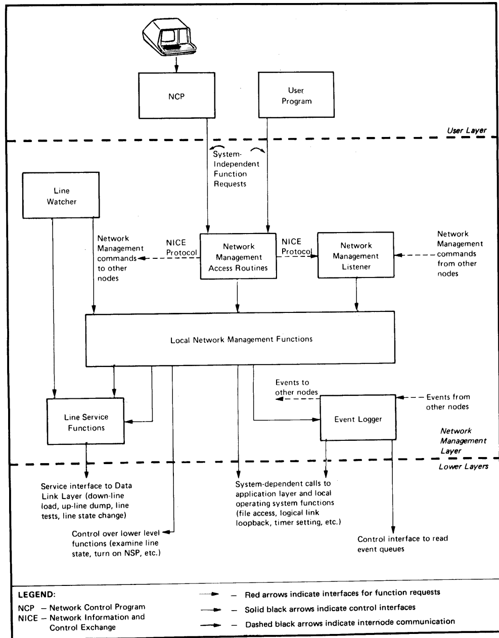
Figure 7-1 shows the interrelationship of Network Management components in the user and Network Management layers.
