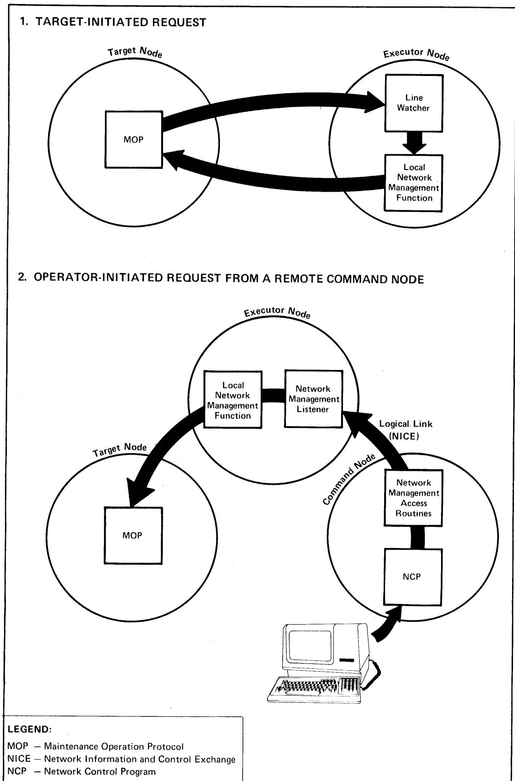
Figure 7-2: Down-Line Load Request Operation
