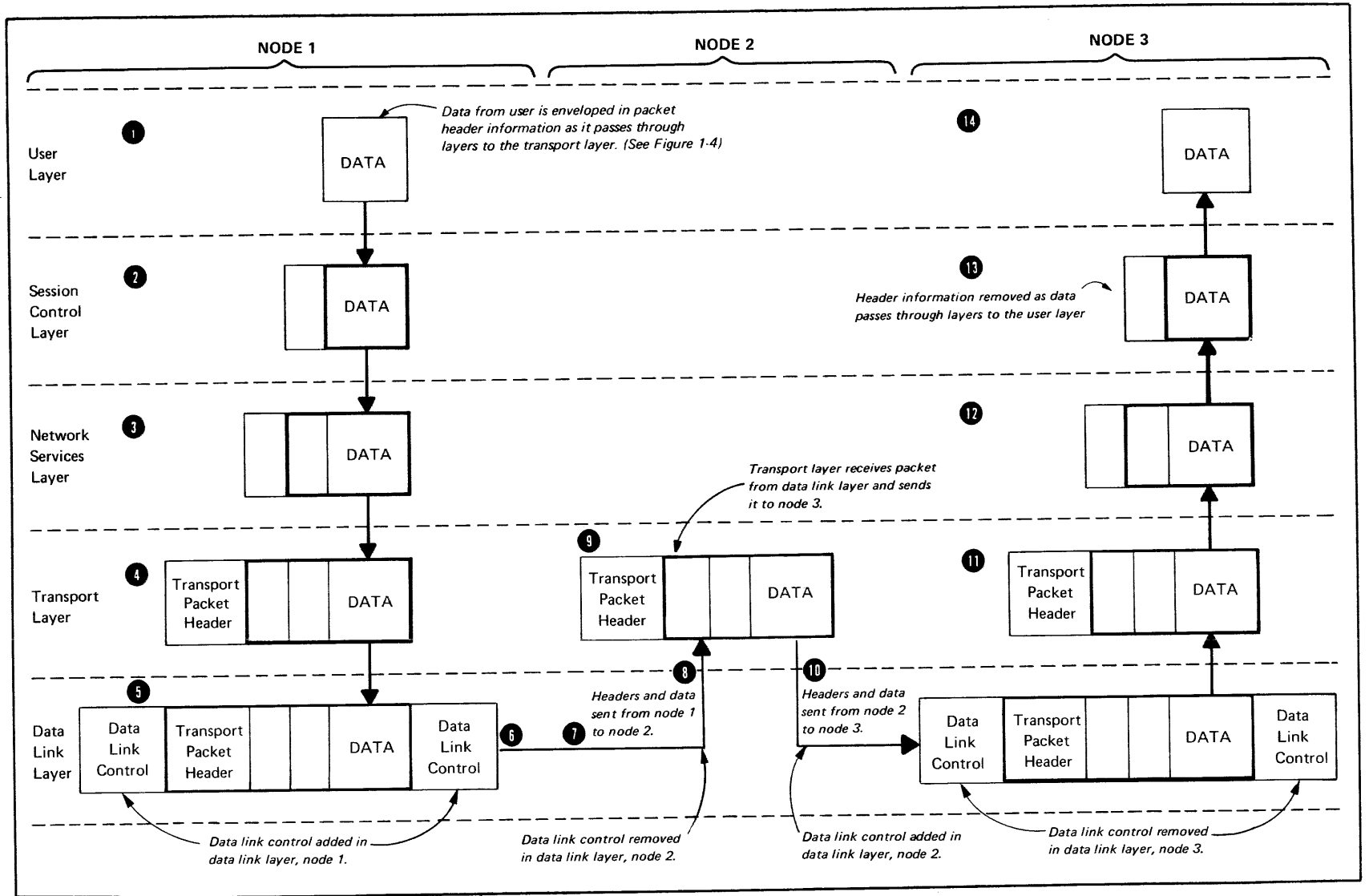
Figure 1-6: Data Flow
