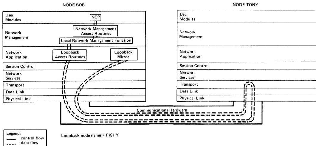
Figure 7-4: Examples of Node Level Testing Using a Loopback Node Name
