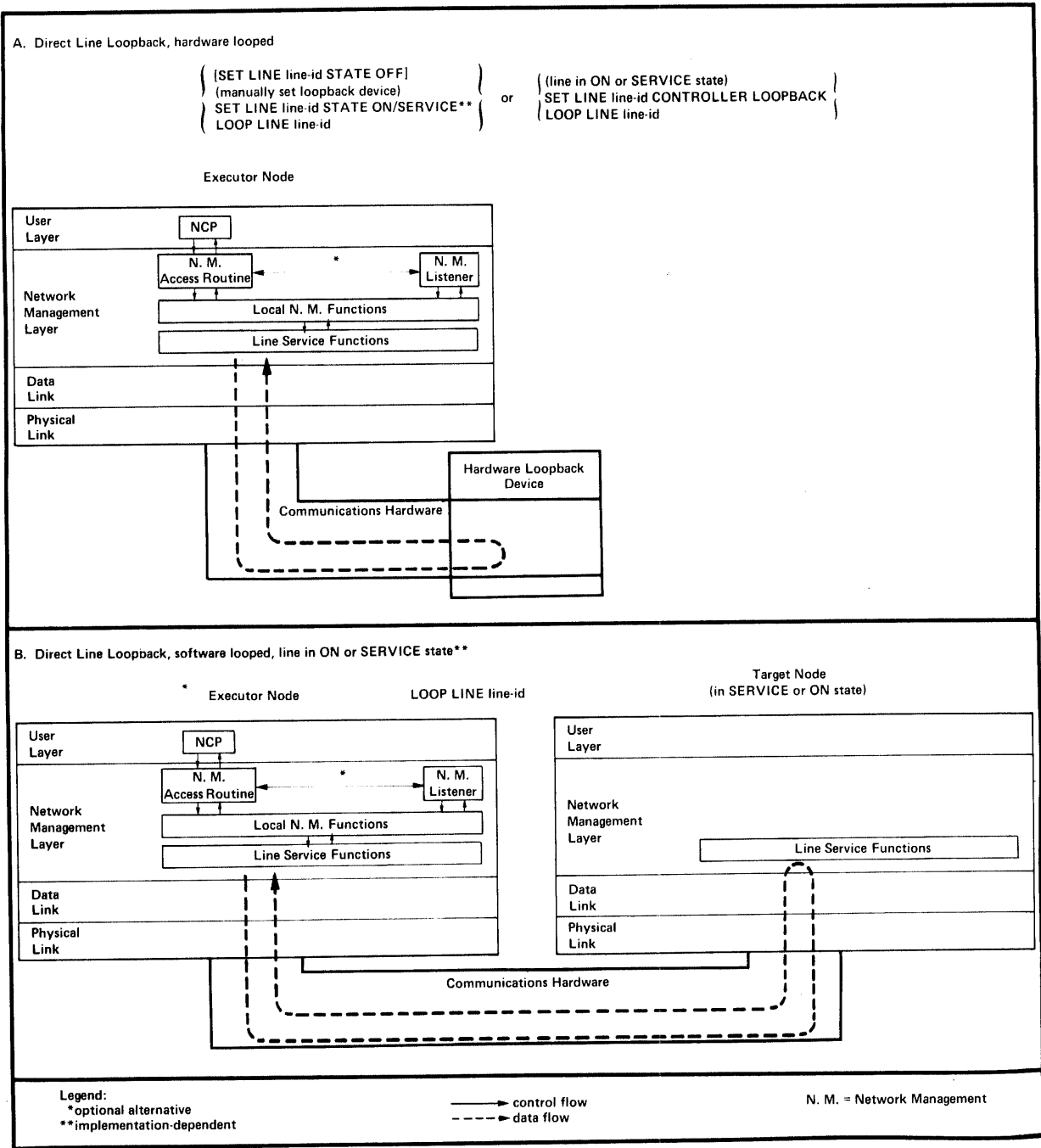
Figure 7-3: Line Loopback Tests
