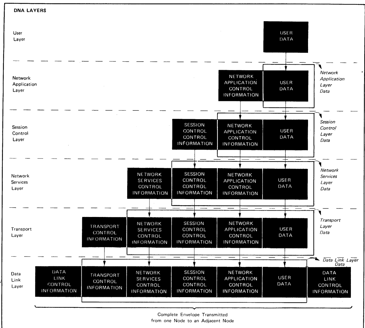
Figure 1-5: Building of Information as Data Passes Through the DNA Layers
